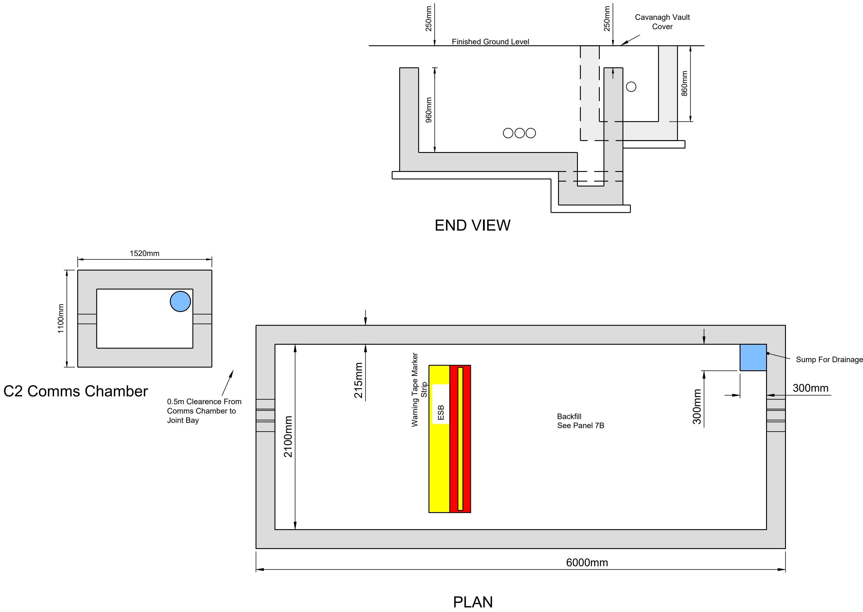
SINGLE CIRCUIT JOINT BAY Scale 1:25
